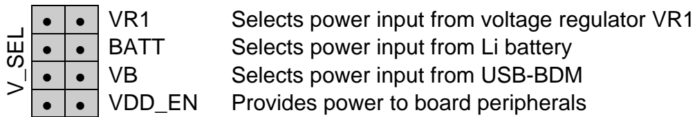
Figure 4: V_SEL Option Header
