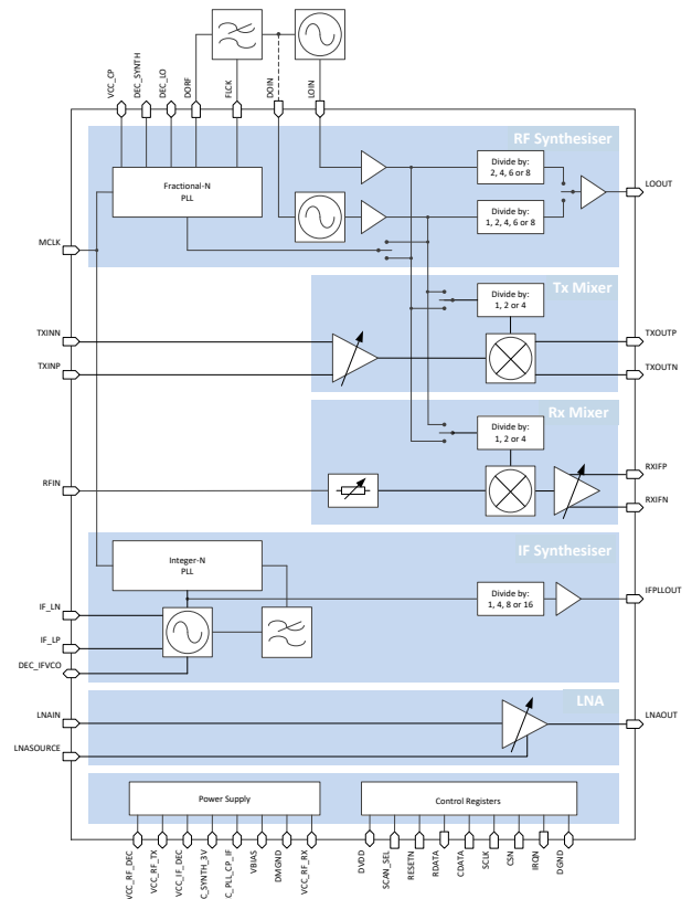
CMX975Q4 Block Diagram
