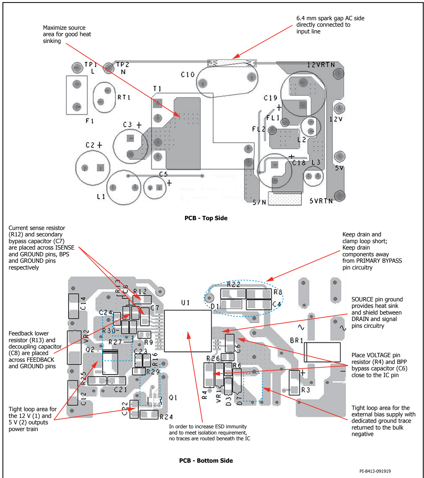
Figure 17. PCB.
