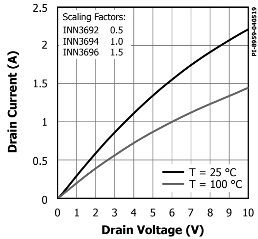
Figure 29. Output Characteristics.
