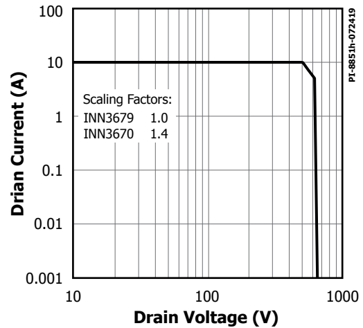
Figure 36. Maximum Allowable Drain Current vs. Drain Voltage (PwGaN Devices INN3679-INN3670).
