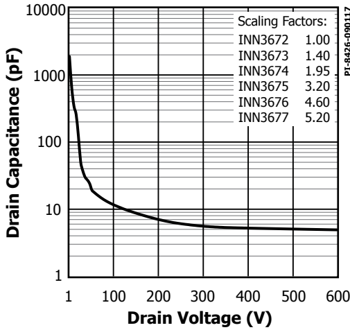
Figure 23. C_{OSS} vs. Drain Voltage.
